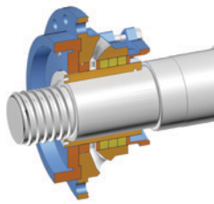
Throat Bushing
