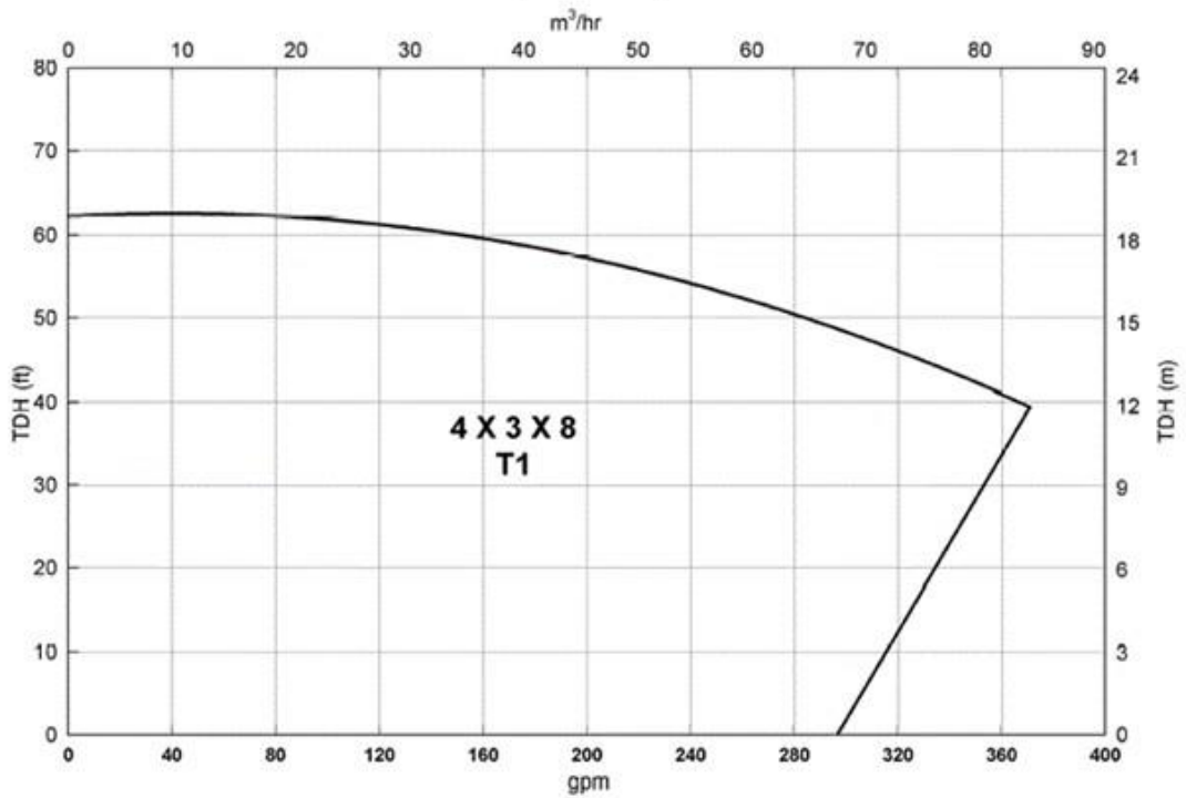
TEIKOKU FAMILY CURVE, 60Hz (1750 RPM)
